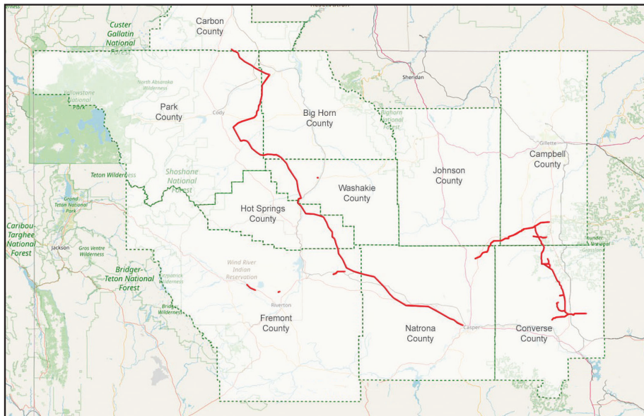
Crude pipeline diameter: 10", 12" and 16"
